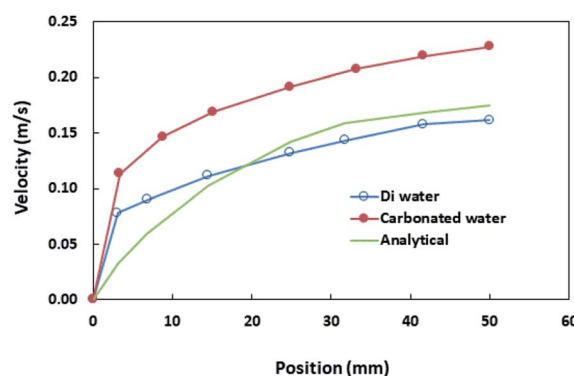
Fig. 3 The translational velocity of distilled and carbonated water droplets. The droplet volume is 40 \mu L and the inclination angle of the surface ( \delta ) is 5°. The analytical solution predicted from eqn (5) is also shown for comparison.
