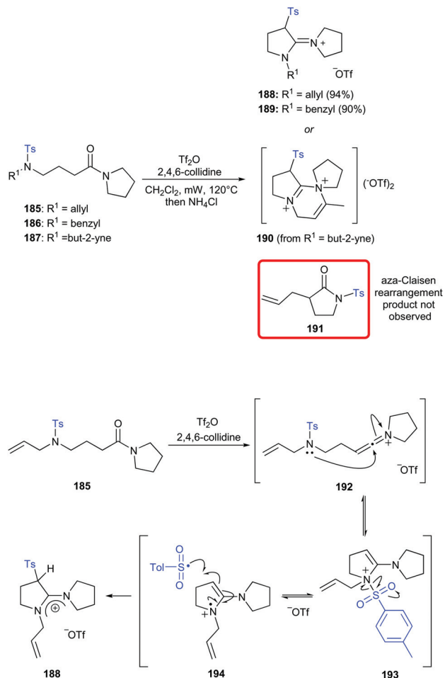
Scheme 26 Generation of amidinium derivatives via 1,3-tosyl migration.
