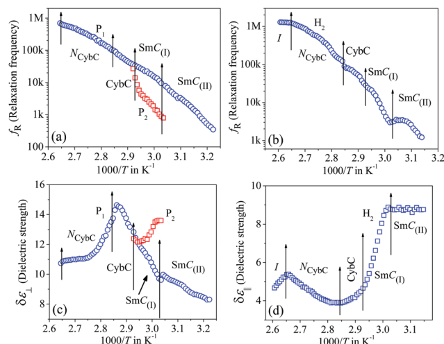
Fig. 5 Temperature dependence of the relaxation frequency ( f_R ) and dielectric strength ( \delta\epsilon' ) for compound 1/10 : (a and c) in planar and (b and d) homeotropic configurations, respectively. Vertical arrows define the corresponding phase-transition temperatures.
