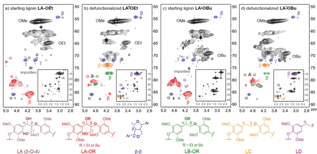
Fig. 8 2D-HSQC NMR spectra (600 MHz, CDCl 3 ) of the linkage region of (a) \alpha -ethoxylated lignin (starting lignin), (b) defunctionalized \alpha -ethoxylated lignin, (c) \alpha -butoxylated lignin (starting lignin), and (d) defunctionalized \alpha -butoxylated lignin; defunctionalized lignins were obtained by dehydrogenative decarbonylation; reaction conditions: 200 mg LA-OEt or LA-OBu with [\text{Ir}(\text{cod})\text{Cl}]_2 13.4 wt%, rac -BINAP 24.9 wt%, LiCl 3.4 wt% and a drop of water dissolved in 2.5 mL diethyl carbonate reacting at a set temperature of 205 °C for 48 hours.
