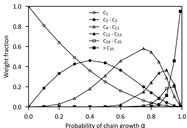
Fig. 20 Anderson–Schulz–Flory distribution: weight fraction of different carbon number products as a function of the chain growth \alpha . \alpha is among other things influenced by the catalyst, the reaction conditions, the temperature and the syngas stoichiometry. Adapted from ref. 351–353.
