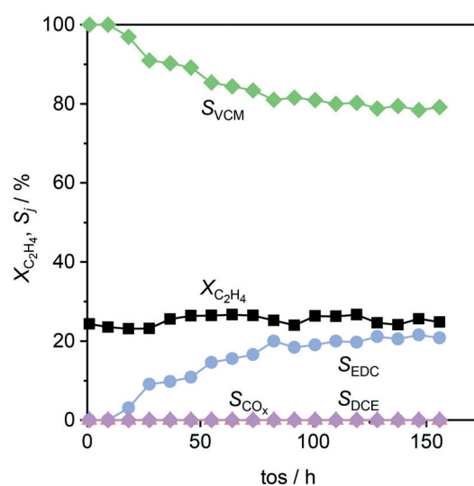
Fig. 10 Conversion and selectivity as a function of time-on-stream in ethene oxychlorination over a CeO_2/ZrO_2 - Ca-I/Al_2O_3 system as depicted in the fourth panel of Fig. 9. Conditions are detailed in Table 2.
