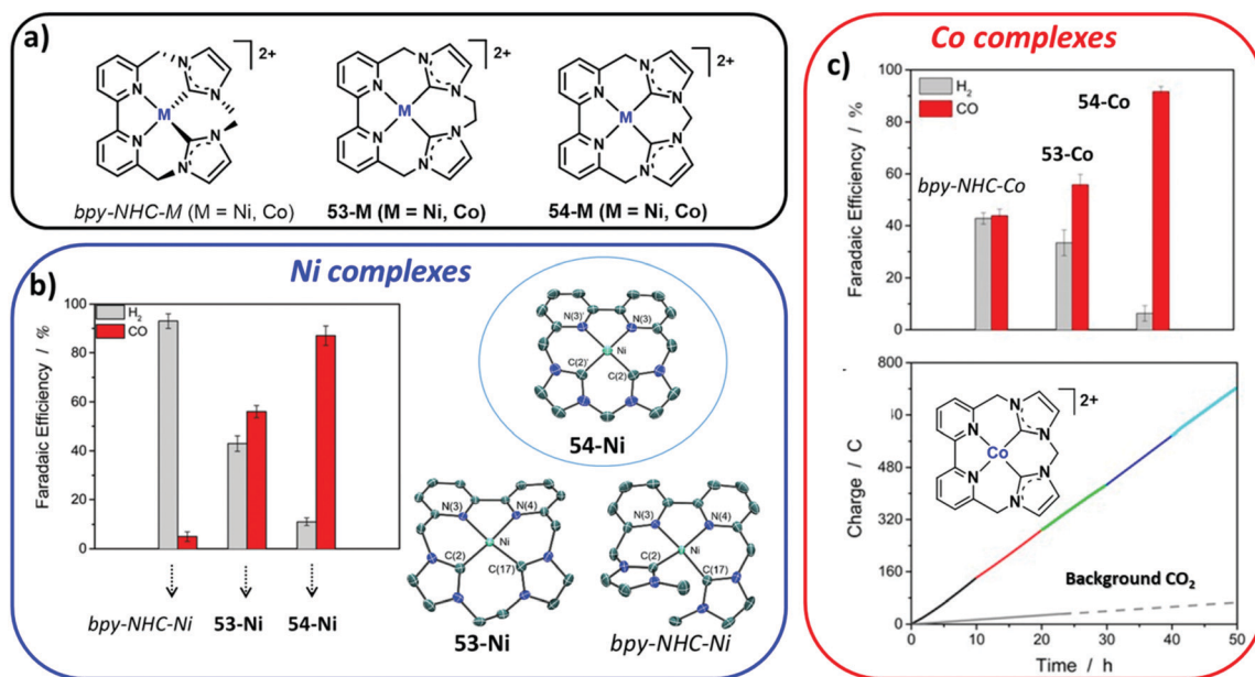
Fig. 17 (a) Sketch of the families of Ni^{II} and Co^{II} catalysts supported by non-macrocylic and macrocylic bipyridyl-NHC ligands. (b) FEs for H_2 (grey) and CO (red) obtained during controlled-potential electrolysis with 0.2 mM of 53-Ni , 54-Ni , bpy-NHC-Ni , respectively. Electrolyte: CO_2 -saturated CH_3CN/0.1 M n-Bu_4NPF_6 solutions containing 2% H_2O at a GC rod. The inset shows the ORTEP diagrams of cations in 53-Ni , 54-Ni and bpy-NHC-Ni . (c) (top) FEs of H_2 (grey) and CO (red) from electrolysis experiments with 10 \mu M Co catalyst in CO_2 -saturated H_2O/0.1 M NaClO_4 at a Hg pool (4 cm dia.) working electrode. On the bottom, a charge vs. time plot of consecutive CPEs is reported with 10 \mu M 54-Co (see inset) in CO_2 -saturated aqueous 0.1 M NaClO_4 . Conditions: E_{appl} = -1.04 V vs. NHE, Hg pool. CO_2 was re-saturated every 10 h. Adapted with permission from ref. 258 and 259. Copyright 2018–2019 Royal Society of Chemistry and American Chemical Society, respectively.
