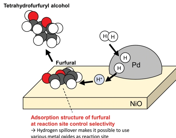
Fig. 3 Selective hydrogenation of furfural over \text{NiO} using hydrogen spillover from \text{Pd} .
