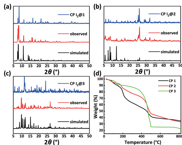
Fig. 4 PXRD patterns of CPs: (a) 1, (b) 2, and (c) 3 and (d) TGA diagrams of CPs 1–3.
