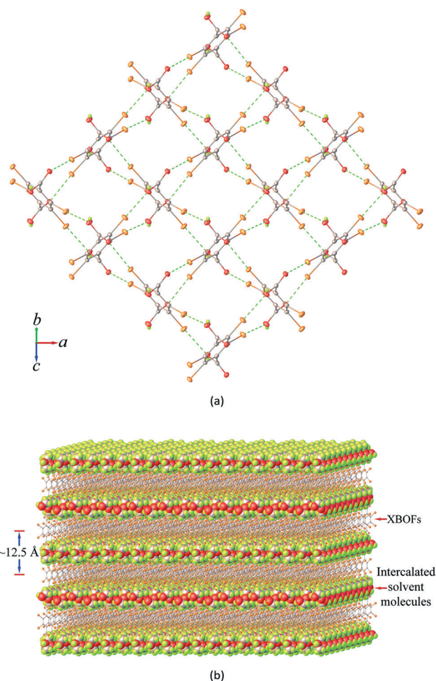
Fig. 1 Perspective view of 1EG as representative showing (a) the 2D halogen-organic frameworks constructed by the Br \cdots O halogen bonding interactions (green dashed lines) and (b) the 3D supramolecular structure.
