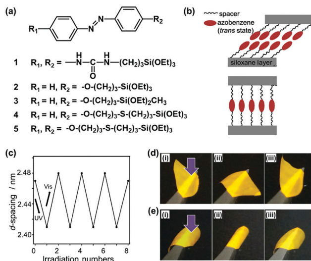
Fig. 4 Soft layered materials based on organopolysiloxane with photomechanical properties. 66–69 (a) Molecular structures of organosiloxanes 1 – 5 . (b) Schematic illustration of the layered structures derived from the organosiloxanes 4 (upper) and 5 (lower) after hydrolyzation and spin-coating on substrate. (c) Microscopic reversible variation of the interlayer distance, namely d -spacing on the X-ray diffraction pattern, with irradiation of UV and visible lights on the thin-film derived from organosiloxane 4 . (d) and (e) Macroscopic bending and unbending behaviors of a free-standing film derived from the mixture of the organosiloxanes 4 and 5 with UV-vis irradiation from the upper (d) and reverse (e) sides. Reprinted with permission from ref. 66. Copyright 2020 American Chemical Society.
