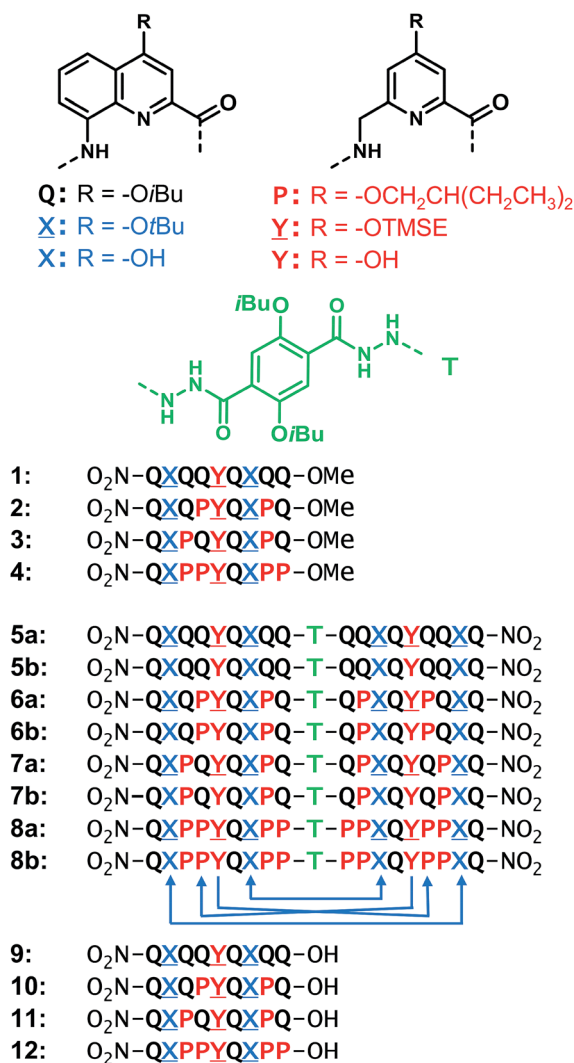
Fig. 1 Structures of units Q , X , P , Y , T and foldamer sequences. X and Y are the protected precursors of hydrogen bonding units X and Y . All flexible units P , Y , or Y are shown in red. Sequences are labelled 'a' when protected and 'b' when deprotected. Sequences end with 8-nitro groups; this group is noted in the replacement of the NH group at terminal Q units. The T unit constitutes an inversion of C → N sequence polarity; sequences that contain T thus have two N termini. The arrows below 8b indicate the hydrogen bonds pattern between the helices. TMSE = 2-trimethylsilylethyl.
