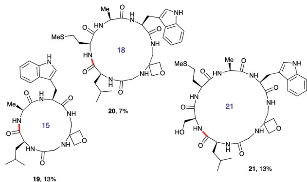
Fig. 4 Additional oxetane modified macrocycles made using SPSS. a,b a Overall yield from first resin-bound amino acid including final RP-HPLC purification. For full details, see ESI. † b Bond formed in macrocyclisation indicated in red.
