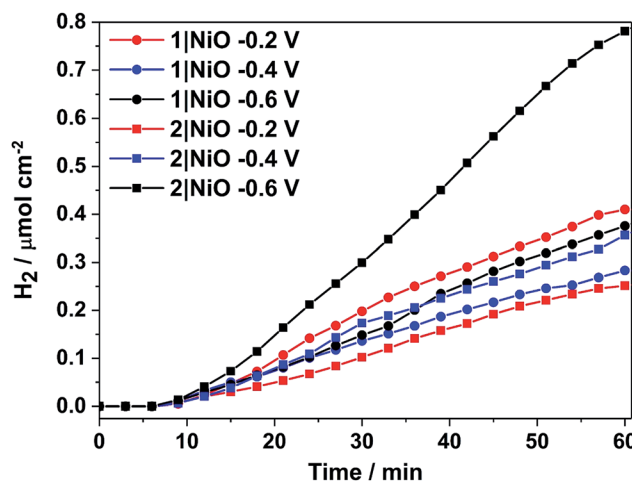
Fig. 8 Cumulative photoelectrocatalytic \text{H}_2 production by 1|NiO and 2|NiO during the chronoamperometry measurements at different E_{\text{appl}} (Fig. 7 and S3 in the ESI†). Chopped light illumination was applied during the first 10 min followed by constant light illumination until the end of the measurement ( \text{AM1.5} , 100 \text{ mW cm}^{-2} ).
