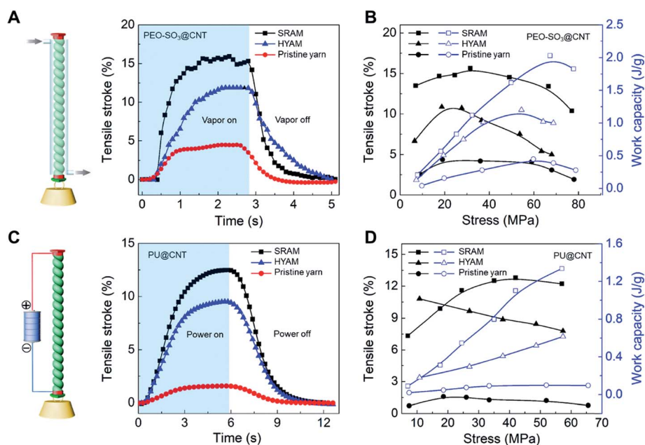
Fig. 26 Isobaric tensile actuation of self-coiled, sorption-powered and electrothermally powered SRAMs, HYAMs, and pristine CNT yarns. (A) Tensile stroke vs. time for a \text{PEO-SO}_3\text{@CNT} SRAM and HYAM and a pristine yarn when actuated by ethanol absorption using the configuration shown on the left and a stress of 33 \text{ MPa} . Sorption was from a near-equilibrium ethanol concentration in dry air and desorption was by dynamic pumping. Before coiling, the diameters of the \text{PEO-SO}_3\text{@CNT} SRAM and HYAM and the pristine yarn were 43 , 47 , and 38 \mu\text{m} , respectively. (B) Tensile stroke and contractile work capacity vs. applied stress for the sorption-actuated muscles of (A). (C) The time dependence of the tensile stroke for a \text{PU@CNT} SRAM and HYAM and a pristine CNT yarn when electrothermally actuated under 42 \text{ MPa} stress using 0.25 \text{ W cm}^{-1} power, which provided temperatures of 85 , 93 , 97^\circ\text{C} , respectively. The device structure is shown on the left. Before coiling, the diameters of the \text{PU@CNT} SRAM and HYAM and the pristine yarn were 65 , 71 , and 51 \mu\text{m} , respectively. (D) Tensile stroke and contractile work capacity vs. applied stress for the electrothermally actuated yarns in (C). This figure has been reproduced from ref. 9 with permission from AAAS.
