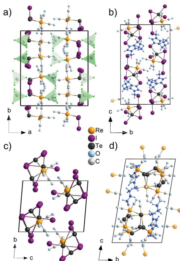
Fig. 1 Unit cells of the Te–Re carbonyls: (a) [\text{TeI}_2\text{Re}(\text{CO})_5][\text{AlCl}_4] ( 1 ); (b) [\text{BMIm}][\text{Te}_2\text{I}_4(\mu\text{-I})_2\text{Re}(\text{CO})_4] ( 2 ); (c) \{\text{Te}_3\text{I}_2(\mu\text{-I})_3(\mu_3\text{-I})\}\text{Re}(\text{CO})_4 ( 3 ); (d) [\text{BMIm}][(\text{Te}_2)_3\{\text{Re}(\text{CO})_3\}_2\{\text{Re}(\text{CO})_4\}_3] ( 4 ) [\text{BMIm}]^+ displayed in dark blue, [\text{AlCl}_4]^- displayed in light green.
