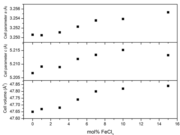
Fig. 5 Variation of cell parameters a , c and cell volume of the films with a change of mol% \text{FeCl}_3 added to the precursor solution. The increase of cell parameters confirms the incorporation of Cl into the ZnO lattice.
