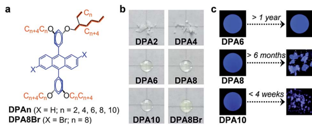
Fig. 1 (a) Chemical structures of \text{DPA}_n ( n = 2, 4, 6, 8 , and 10 ) and \text{DPA8Br} . (b) Photographs of freshly synthesized \text{DPA}_n and \text{DPA8Br} in daylight at 20 °C, with a drop of fluid or powder of solid on a glass plate. (c) Photographs of \text{DPA6} , \text{DPA8} , and \text{DPA10} as fresh (left) and after long-term of aging at ambient temperature (right) taken under irradiation of a UV lamp (365 nm).
