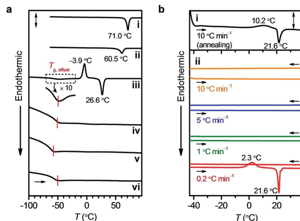
Fig. 2 (a) DSC thermograms of (i) \text{DPA2} , (ii) \text{DPA4} , (iii) \text{DPA10} , (iv) \text{DPA8} , (v) \text{DPA8} , and (vi) \text{DPA8Br} during the first heating scan from -100 to 95 °C at 10 °C \text{min}^{-1} under \text{N}_2 flow ( T_{g, \text{offset}} the offset temperature of the glass-to-isotropic liquid transition; scale bar (sb), 2.0 \text{W g}^{-1} for (i–iii) and 0.2 \text{W g}^{-1} for (iv–vi)). (b) DSC thermograms of \text{DPA8} (i) during the heating scan from -45 to 40 °C at 10 °C \text{min}^{-1} after annealing at -45 °C for 12 h (sb, 0.1 \text{W g}^{-1} ) and (ii) during the heating/cooling cycles between -45 and 40 °C at 10 °C \text{min}^{-1} (orange; sb, 1.6 \text{W g}^{-1} ), 5 °C \text{min}^{-1} (blue; sb, 1.6 \text{W g}^{-1} ), 1 °C \text{min}^{-1} (green; sb, 0.4 \text{W g}^{-1} ), and 0.2 °C \text{min}^{-1} (red; sb, 0.1 \text{W g}^{-1} ) under \text{N}_2 flow.
