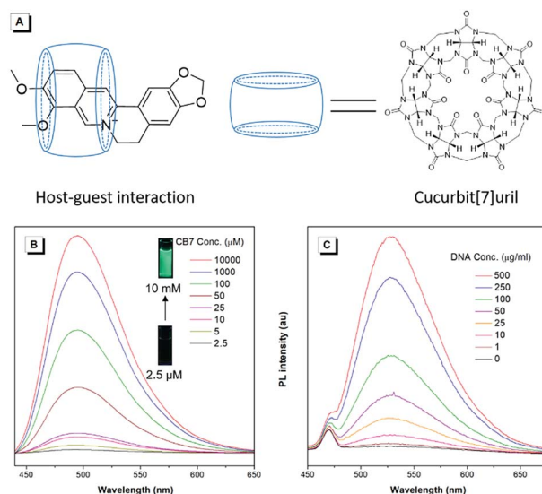
Fig. 4 (A) Schematic illustration of host–guest interactions between BBR chloride and cucurbit[7]uril (CB7). (B) PL spectra of BBR chloride in cucurbit[7]uril (CB7) aqueous solution with different concentrations. Slit width: 4 nm. (C) PL spectra of BBR chloride in bovine thymus DNA aqueous solution with different concentrations. Slit width: 5 nm. Excitation wavelength: 405 nm.
