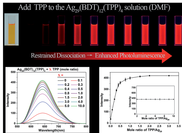
Fig. 4 PL variation trend of the Ag 29 (BDT) 12 (TPP) 4 NC resulting from the addition of different molar ratios of TPP ligand. (Top) PL intensity variation monitored by digital photography of the Ag 29 (BDT) 12 (TPP) 4 NC in the solution state under UV light. (Bottom-left) PL intensity variation monitored using the fluorescence spectrometer. (Bottom-right) PL intensity variation monitored at the fixed point of 642 nm.
