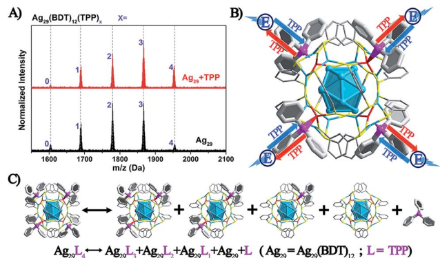
Fig. 3 (A) ESI-MS spectra of the Ag 29 (BDT) 12 (TPP) 4 NC with or without the addition of TPP. (B) Illustration of the dynamic TPP dissociation–aggregation process on the Ag 29 (BDT) 12 (TPP) 4 and the corresponding energy loss. (C) The dynamic TPP dissociation–aggregation reversible reaction. Color codes: cerulean/red spheres, Ag; yellow spheres, S; purple spheres, P; grey spheres, C; white spheres, H.
