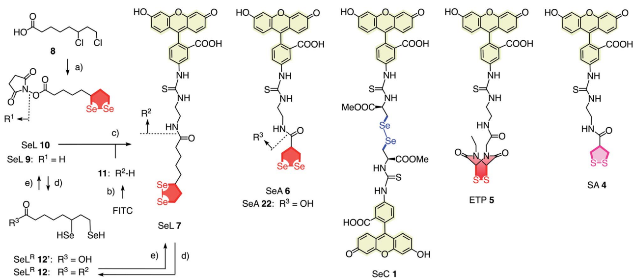
Fig. 2 Complete structure of all transporters used (neutral form), with representative synthesis and reduction for SeL 7 . (a) (1) Several steps, ref. 17, (2) NHS, DCC, THF, rt, 18 h, 53%; (b) several steps, ref. 1; (c) DMF, rt, 3 h, 14%; (d) TCEP, <5 min; (e) air.
