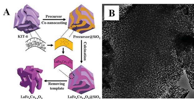
Fig. 1 (A) Synthesis process of the mesoporous LaFe x Co 1-x O 3 perovskite oxides by co-nanocasting process using mesoporous KIT-6 as a hard template, (B) the as-prepared mesoporous LaFeO 3 . Reproduced with permission from ref. 34. Copyright© 2013, Royal Society of Chemistry.
