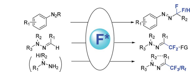
Fig. 2 Different methods for synthesis of fluorinated hydrazones.
