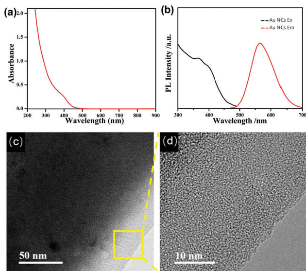
Fig. 1 UV-vis absorption spectrum (a), photoexcitation ( \lambda_{em} = 565 nm, black line) and photoemission ( \lambda_{ex} = 365 nm, red line) spectra of the Au NCs (b). (c) TEM image of the Au NCs at pH 2.0. (d) HRTEM image of the zone marked by the yellow frame in (c).
