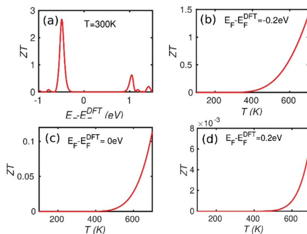
Fig. 5 (a) The thermoelectric figure of merit at 300 \text{ K} for the structure shown in Fig. 1(b). (b)–(d) The thermoelectric figure of merit as a function of temperature for three particular Fermi energies ( E_F - E_F^{\text{DFT}} = -0.2 \text{ eV} , E_F - E_F^{\text{DFT}} = 0 \text{ eV} , E_F - E_F^{\text{DFT}} = 0.2 \text{ eV} ) for the structure shown in Fig. 1(b). These calculations are valid provided the forces entering the phonon dynamical matrix are harmonic. Anharmonic effects are negligible, provided the temperature does not approach the melting point of the material. The melting point of \text{MoS}_2 is greater than 1400 \text{ K} and therefore we have restricted our analysis to approximately half that value.
