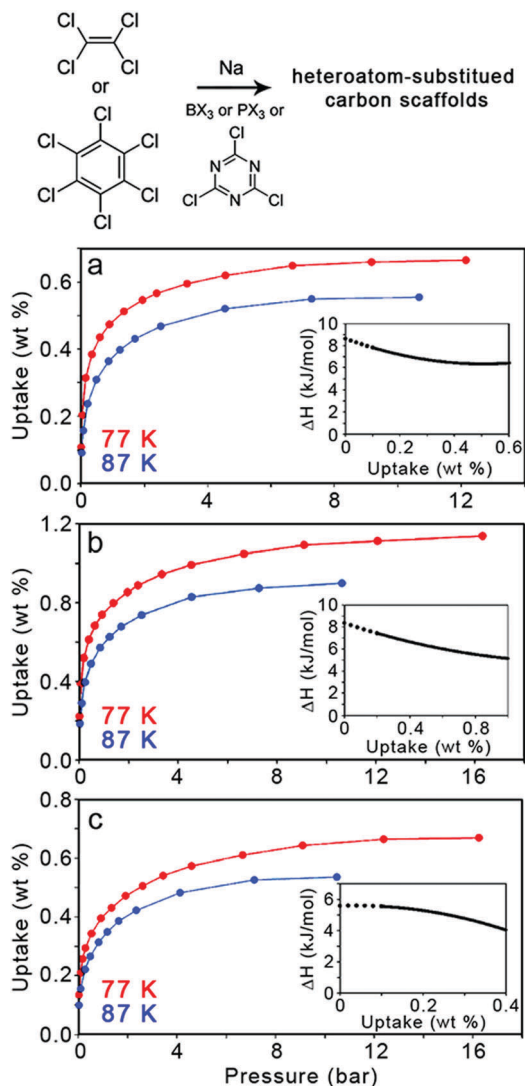
Fig. 14 (top) Bottom-up synthesis of heteroatom-substituted carbons; reaction conditions: tetrachloro-substituted aromatic compounds, X = \text{halogen or OR} , and temperatures between 250 and 350 °C. (bottom) Hydrogen uptake at 77 and 87 K for (a) boron-, (b) phosphorus-, and (c) nitrogen-substituted carbons. Adapted with permission from Z. Jin, Z. Z. Sun, L. J. Simpson, K. J. O'Neill, P. A. Parilla, Y. Li, N. P. Stadie, C. C. Ahn, C. Kittrell and J. M. Tour, J. Am. Chem. Soc. , 2010, 132 , 15246. Copyright 2008 American Chemical Society.
