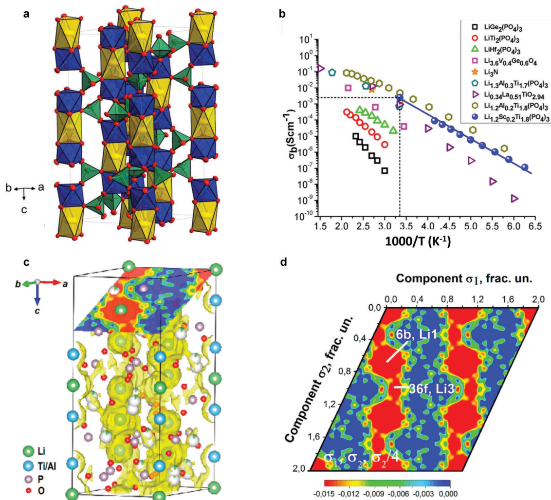
Fig. 5 (a) Unit cell (space group R\bar{3}c ) of \text{LiTi}_2(\text{PO}_4)_3 . Yellow elongated octahedra ( M_1/6b ) are occupied by \text{Li}^+ ; blue octahedra ( M_2/12c ) are occupied by \text{Ti}^{4+} ; and green tetrahedra are occupied by \text{P}^{5+} (18e); \text{O}^{2-} is located at the corners of the polyhedra (small red circles, two Wyckoff positions 36f). 118 (b) Ion conductivity of NaSICON structured Li ion solid electrolytes. 134 (c) MEM-reconstructed negative nuclear density maps. 52 (d) Sections of bond-valence mismatch and negative nuclear densities \text{Li}_{1.3}\text{Al}_{0.3}\text{Ti}_{1.7}(\text{PO}_4)_3 . 52 Reproduced with permission from ref. 52, 118, 134. Copyright (2016, 2017) American Chemical Society.
