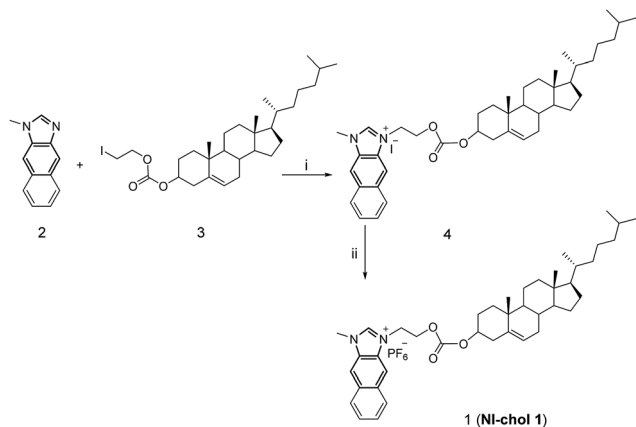
Scheme 1 The synthetic procedure of NI-cholesterol 1 . (i) Acetonitrile, N_2 , reflux, 24 h, 81.1%; (ii) DMF, KPF_6 , 98.6%.
