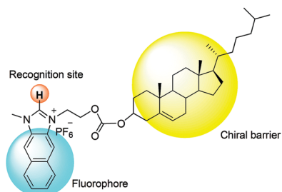
Fig. 1 Design strategy of NI-cholesterol 1 .
