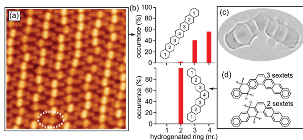
Fig. 3 (a) STM image ( U = 1.7 V// = 186 pA) of a full monolayer sample of Br-1 after annealing to 180 °C. The oval marks a tetrahydro-heptacene molecule after a methylene migration (intermediate 1' ). (b) Histograms displaying the occurrence of differently positioned hydrogenated rings (numbered as in the insets of molecular structures) for dihydro intermediates of heptacene (top) and heptaphene (bottom). (c) Laplace-filtered constant-height STM image ( U = 2 mV) of a heptaphene intermediate with a single hydrogenated ring. (d) Schematics revealing the maximized number of Clar sextets for dihydroheptaphene when hydrogenated at the second ring (compared below, e.g. , with hydrogenation at the third ring).
