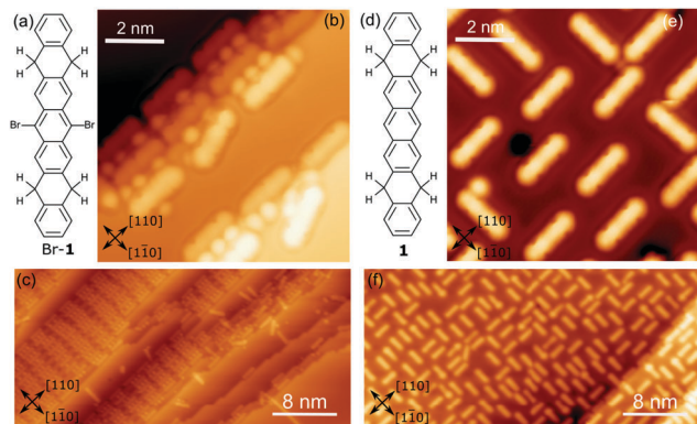
Fig. 1 (a) Chemical structure of precursor Br-1 and representative small (b) and large (c) scale STM images of the surface after its deposition on Ag(001) held at RT [ U = 30 mV// = 70 pA (b) and U = 30 mV// = 100 pA (c)]. (d) Chemical structure of reactant 1 and representative small (e) and large (f) scale STM images of the sample after its deposition on Ag(001) [ U = 35 mV// = 100 pA (e) and U = 600 mV// = 600 pA (f)].
