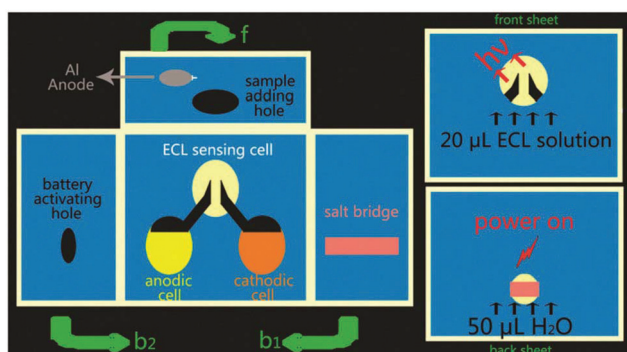
Fig. 36 Schematic diagram of the working principle of a m-s-OECDL. f: Front sheet; b1: the sheet folded to the back first; b2: the back sheet. (Reprinted with permission from ref. 165. Copyright 2013 The Royal Society of Chemistry.)
