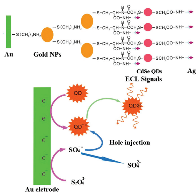
Fig. 7 Schematic illustration of fabrication process (A) and ECL mechanisms (B) of the ECL immunosensor. (Reprinted with permission from ref. 49. Copyright 2008 Elsevier.)
