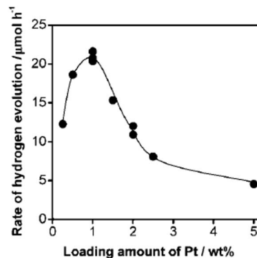
Fig. 4 Dependence of the \text{H}_2 evolution rate, when using Pt-loaded g- \text{C}_3\text{N}_4 under visible light, on the loading amount of Pt. Reprinted with permission from ref. 56. Copyright 2009, American Chemical Society.
