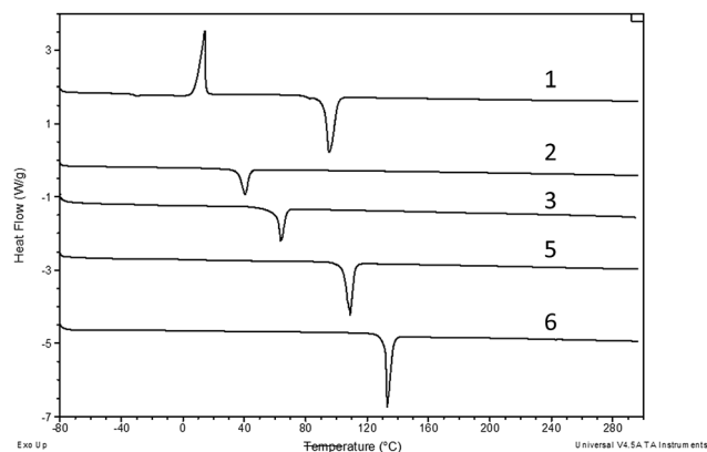
Fig. 4 DSC curves compounds 1–3, 5, 6. Measurements were taken in open pans under nitrogen at ramp rate of 10 °C min -1 . The curves have been offset but not rescaled.
