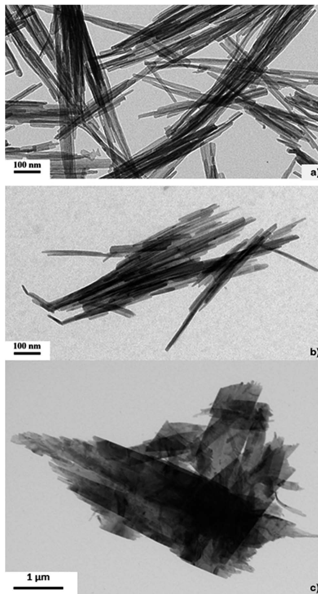
Fig. 2 Bright field TEM image of CuO nanocomposite: (a) with CIL; (b) with CIL r ; (c) without ionic liquid.
