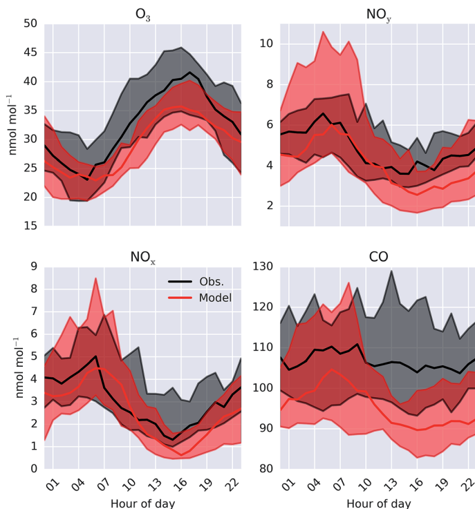
Fig. 3 Modelled ("HAL") and observed median diel mixing ratio at Weybourne of \text{O}_3 , \text{NO}_y , \text{NO}_x and \text{CO} during the observational period. Shaded regions give 25 th and 75 th percentiles.
