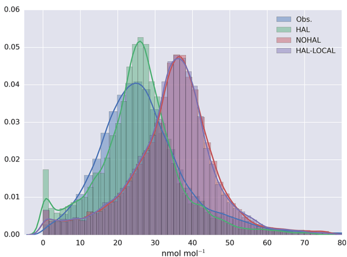
Fig. 4 Probability distribution function of observed and modelled \text{O}_3 mixing ratios at selected UK AURN background sites ( N = 63 ) for the observation period (29 th June to 1 st August 2015). Modelled values are shown for the simulation with halogens ("HAL"), without halogens ("NOHAL"), and with halogens only within the European domain ("HAL-LOCAL").
