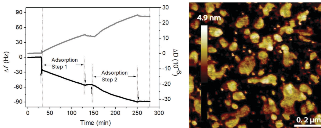
Fig. 9 Left Panel: Adsorption from a solution containing 0.5 mg mL -1 DPPC and 0.5 mg mL -1 hyaluronan (start marked by ↑) on a silica surface in 155 mM NaCl solution at 55 °C monitored by QCM-D (frequency (black line) and dissipation (grey line) change). Rinsing (start marked by ↓) was done with 155 mM NaCl solution at 55 °C. Right panel: AFM topography image of the adsorbed layer formed after 40 minutes of adsorption from solutions containing 0.5 mg mL -1 DPPC and 0.5 mg mL -1 hyaluronan in 155 mM NaCl on a silica surface. After 40 minutes the solution was exchanged with pure 155 mM NaCl solution, and the resulting layer was imaged in this solution at a temperature of 47 °C. Image size 1 × 1 μm 2 . Note that the AFM tip will deform and possibly disrupt the adsorbed aggregates, so the height of these aggregates when undisturbed by the tip is underestimated in the image. Adopted with permission from ref. 11 © 2017 Elsevier Inc.
