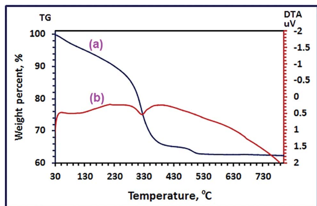
Fig. 6 TG (a), and DTA (b) analyses of the as-prepared \text{CoCO}_3/\text{FeCO}_3 nanocomposite under nitrogen gas.
