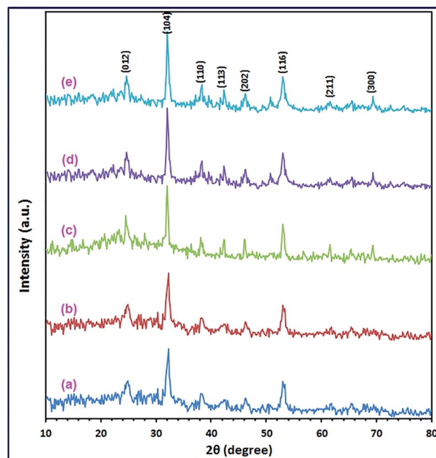
Fig. 3 XRD patterns of the as-synthesized \text{CoCO}_3/\text{FeCO}_3 composites under hydrothermal reactions: \text{Co}^{2+}:\text{Fe}^{2+} : ascorbic acid : \text{CO}_3^{2-} molar ratio of 0.4 : 0.6 : 1 : 3, respectively, at 140 °C, for varying reaction times of 1.5 (a), 3 (b), 6 (c), 12 (d), and 24 h (e).
