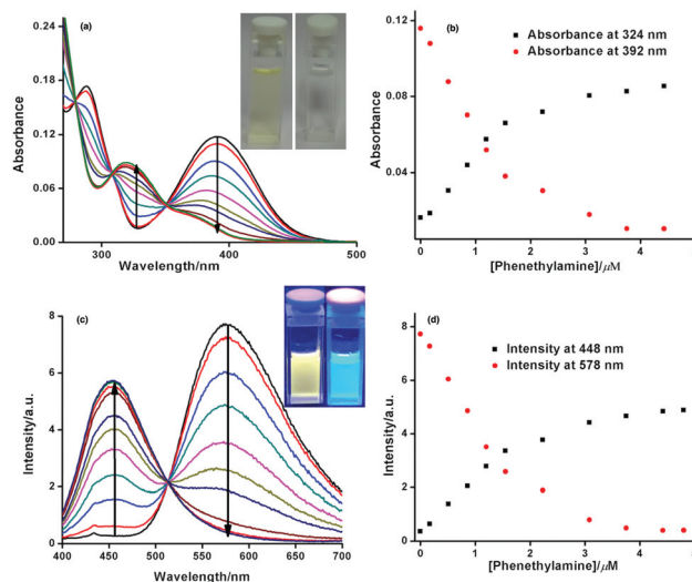
Fig. 2 (a) Titration of ANH with phenethylamine by UV (inset shows digital photograph of ANH solution in DMA before and after the titration). (b) Plot of the change of absorption at two different wavelengths with concentration of phenethylamine. (c) Titration of ANH with phenethylamine using fluorescence by exciting at 385 nm (inset shows digital fluorescence images of ANH solution in DMA before and after the titration). (d) Plot of the change of intensity at two different wavelengths with concentration of phenethylamine.
