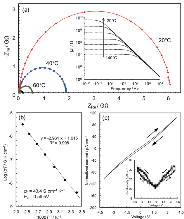
Fig. 3 AC impedance analyses. (a) Complex-plane impedance data for a pellet of 3 (red: 20\text{ }^\circ\text{C} ; blue: 40\text{ }^\circ\text{C} ; green: 60\text{ }^\circ\text{C} ; and black: 80\text{ }^\circ\text{C} ). The inset shows \log|Z| vs. \log frequency plots. (b) Arrhenius plot of the electronic conductivity. (c) Current–voltage characteristics measured by cyclic voltammetry scanned at 10\text{ mV s}^{-1} at 25\text{ }^\circ\text{C} .
