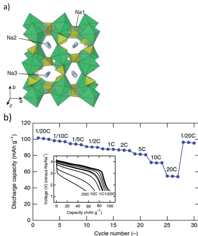
Fig. 8 (a) \text{Na}_2\text{Fe}_2(\text{SO}_4)_3 structure projected along the c axis, and (b) capacity retention upon cycling up to 30 cycles under various rate of \text{C}/20 (2 Na in 20 h) to 20 \text{ C} . Reproduced with permission 80 © 2014, Nature Publishing Group.
