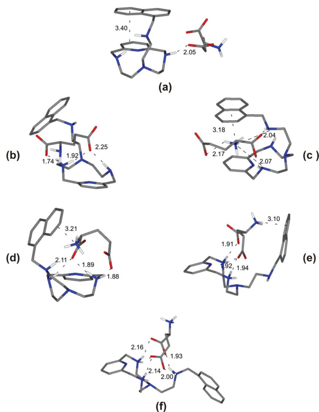
Fig. 4 Minimum energy structures calculated for the complexes [\text{L2-(Glu)}]^{2-} (a), [\text{HL2(Glu)}]^{-} (b), [\text{L2(HGlu)}]^{-} (c), [\text{HL2(HGlu)}] (d), [\text{H}_2\text{L2(HGlu)}]^{+} (e), and [\text{H}_3\text{L2(HGlu)}]^{2+} (f).
