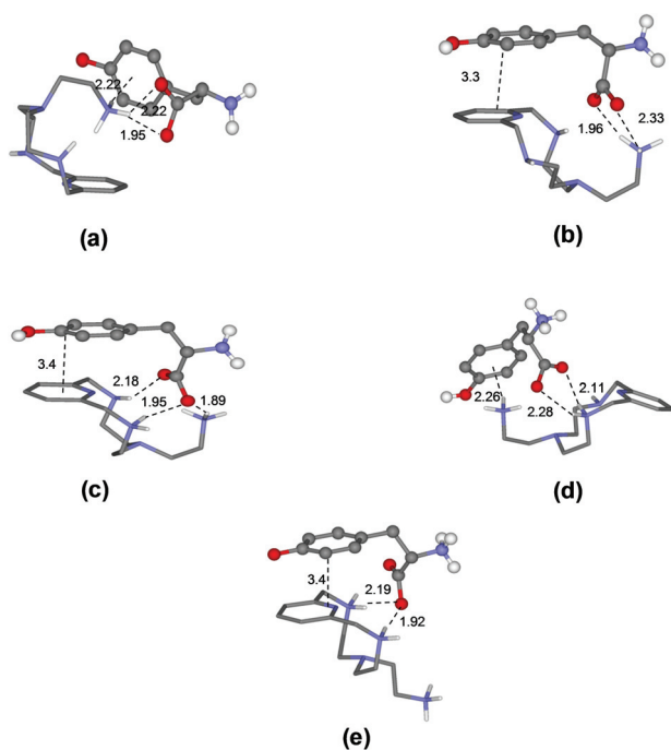
Fig. 3 Minimum energy structures calculated for the complexes [\text{HL1-(Tyr)}]^{-} (a), [\text{HL1(HTyr)}] (b), [\text{H}_2\text{L1(HTyr)}]^{+} (c), [\text{H}_2\text{L1(H}_2\text{Tyr)}]^{2+} (d), and [\text{H}_3\text{L1(H}_2\text{Tyr)}]^{3+} (e).
