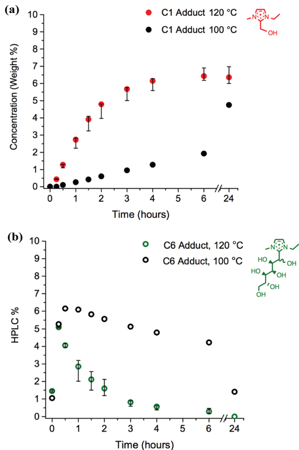
Fig. 10 Comparison of adduct formation for [C_2C_1im][OAc] , 1a + 10 wt% D-(+)-glucose, 12 , heated for 24 hours at 120 and 100 °C: (a) wt% of the C1 adduct, [C_2C_1(HO)C_1^{12}im]^+ ; (b) HPLC% of the intermediate C6 adduct cation.
