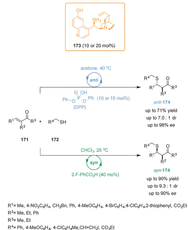
Scheme 52 Solvent- and acid-dependant diastereodivergent Michael addition of alkyl thiols to \alpha,\beta -unsaturated ketones catalyzed by cinchona alkaloid derivative 173 . 98
