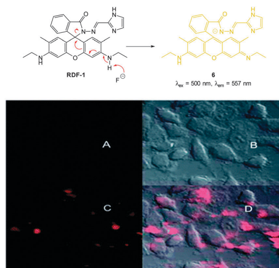
Fig. 6 Top: structure and reaction of rhodamine probe RDF-1 with \text{F}^- . Bottom: (A) fluorescence image of HeLa cells incubated with RDF-1 ; (B) corresponding bright-field image; (C) fluorescence image of HeLa cells incubated with RDF-1 and NaF; (D) overlaid images of HeLa cells (B and C). Image reproduced with permission. 118
