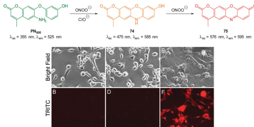
Fig. 73 Top: probe PN600 showing reaction with both \text{ONOO}^- and \text{ClO}^- to form 74 , however only \text{ONOO}^- can oxidise 74 to the red iminoquinone 75 . Bottom: live-cell imaging using PN600 . Phase contrast and fluorescence images of human glioma cells treated with (A, B) PN600 , (C, D) PN600 + \text{ClO}^- , and (E, F) PN600 + SIN-1. Scale = 50 \mu\text{m} . Image reproduced with permission. 290
