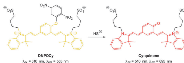
Fig. 50 NIR emissive \text{HS}^- probe DNPOCy .
