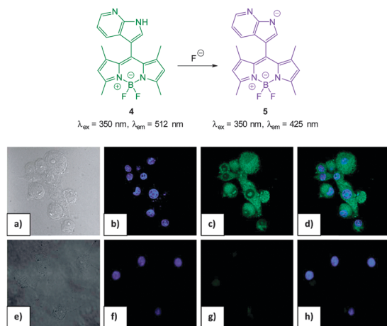
Fig. 5 Top: structure, and deprotonation, of probe 4 by \text{F}^- . Bottom: images of RAW264.7 cells. (a) Bright field image; (b) nuclei stained with 4',6-diamidino-2-phenylindole (DAPI); (c) cells treated with probe 4 ; (d) overlay image of (b) and (c); (e) bright field image of probe 4 and \text{F}^- ; (f) probe 4 and \text{F}^- (g) nuclei with DAPI; (h) overlapping image of (f) and (g). Image reproduced with permission. 115
