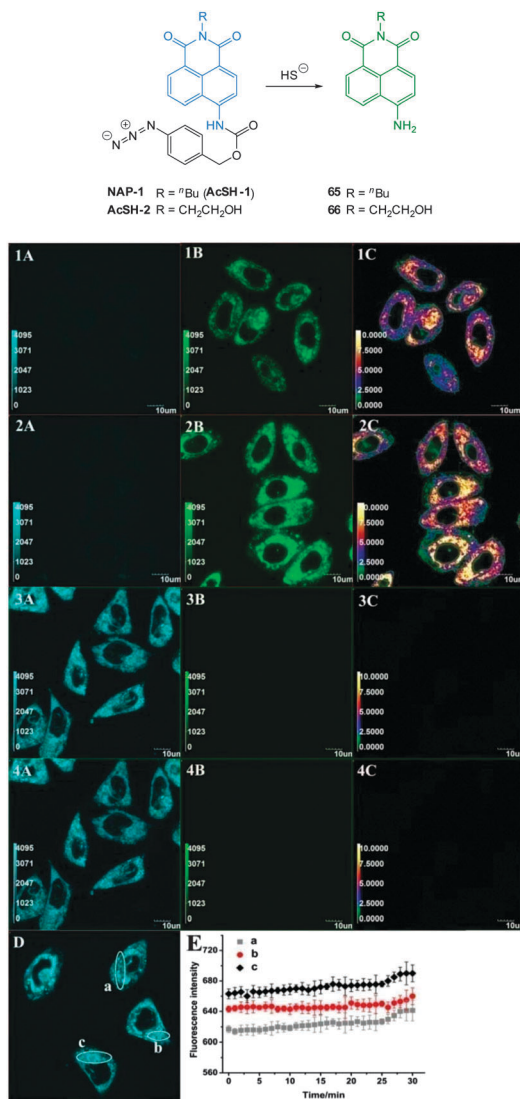
Fig. 63 Confocal fluorescence images of endogenous \text{HS}^- in living MCF-7 cells with NAP-1 . Cells were pre-stimulated with SNP, then with NAP-1 (1A, 1B, 1C). Cells were pre-stimulated with SNP, and then with NAP-1 (2A, 2B, 2C). Cells were pre-treated with \text{DL} -propargylglycine (PPG), and then with NAP-1 (3A, 3B, 3C). Cells in (3A, 3B, 3C) were thereafter treated with SNP (4A, 4B, 4C). Cells were incubated with NAP-1 alone (D). The average fluorescence intensity from the regions of interest a, b and c in (D) was recorded with 60 s intervals (E) ( n = 3 ). Ratiometric images ( F_{530}/F_{468} ) generated by the Olympus software (1C, 2C, 3C, 4C). Scale bars = 10 \mu\text{m} . Image reproduced with permission. 235
