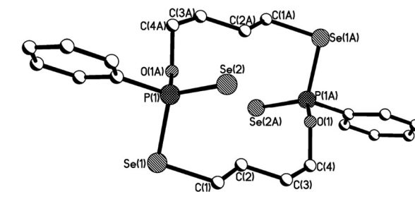
Fig. 4 Crystal structure of 11b ( R,S isomer of 11 ).
