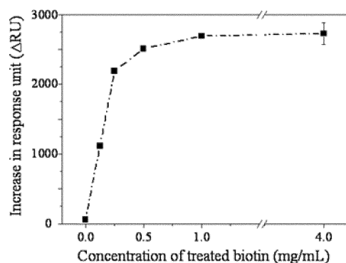
Fig. 2 Binding level of streptavidin on the dendrimer monolayer that had been biotinylated with various concentrations of succinimidyl \alpha -biotin.
