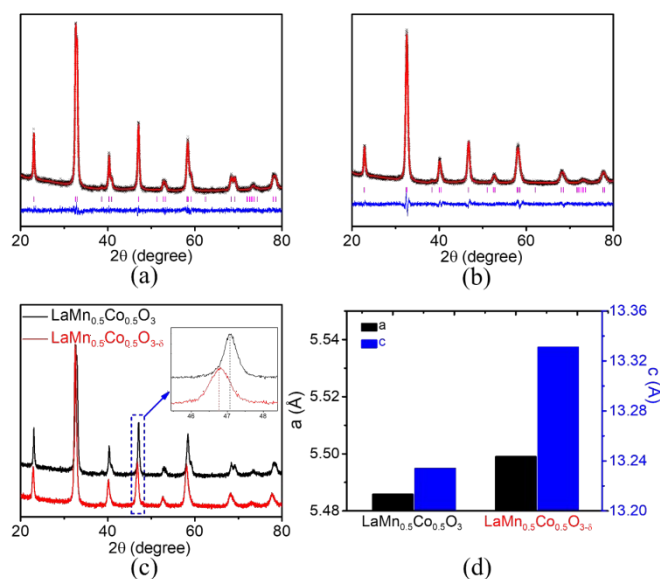
Figure 2. Rietveld refinement profiles for powder X-ray diffraction (PXRD) data of (a) LaMn 0.5 Co 0.5 O 3 and (b) LaMn 0.5 Co 0.5 O 3-δ . (c) Comparison of PXRD data, indicating the peak shift. (d) Comparison of the unit cell dimensions a (black) and c (blue).
