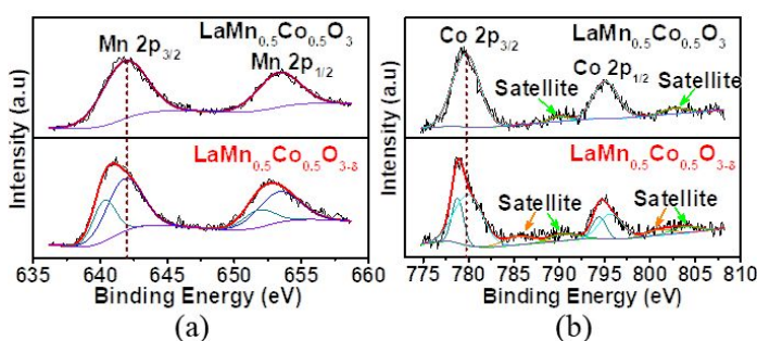
Figure 3. XPS spectra of (a) Mn 2p and (b) Co 2p, showing LaMn 0.5 Co 0.5 O 3 data in the top panel and LaMn 0.5 Co 0.5 O 3-δ at the bottom.
