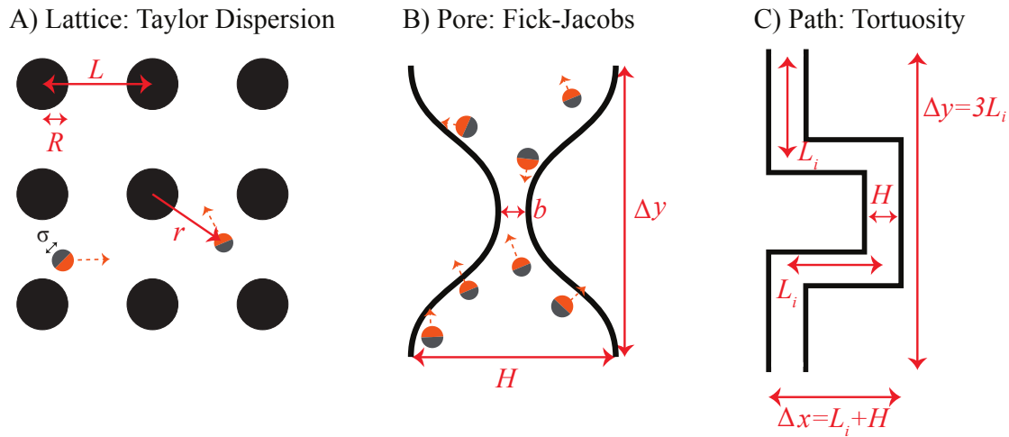
Fig. 1 Diagrams of the three sample systems used to probe diffusivity models. A) An infinite lattice of hard spheres, used to study generalized Taylor dispersion theory. B) A narrow pore of varying constriction, used to probe Fick-Jacobs approximations. C) A winding path, used to test the applicability of tortuosity relations.
