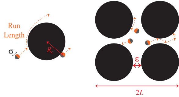
Fig. 2 Diffusivity of swimmers in a lattice array depends strongly on the obstacle density. A) At high porosity, diffusivity decreases linearly with obstacle area density \phi . The radius of the disk is defined as the volume excluded to the ABP R_c = R_{disk} + \sigma/2 . In all our results, we keep \sigma constant and simplify notation by R = R_c . B) At dense packing, ABPs are trapped in small pockets with narrow escape domains of size \epsilon . The lattice is made of disks centered in a unit cell of length L .
