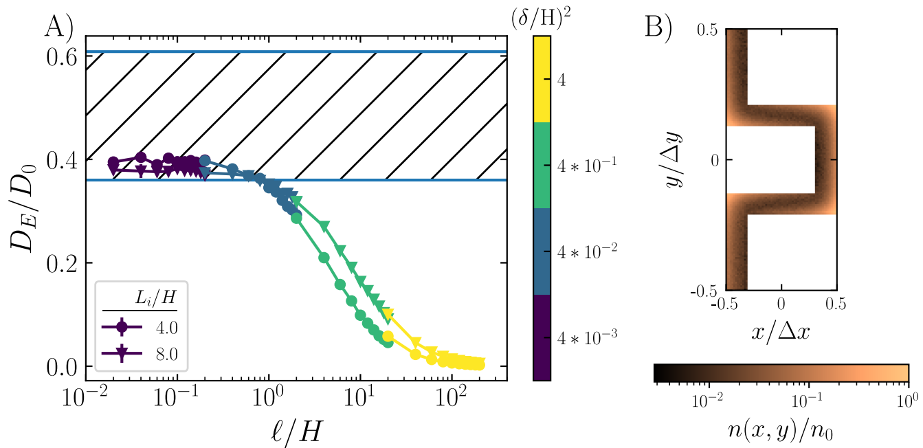
Fig. 8 Tortuosity scalings fail as run length increases beyond the channel width. Brownian dynamics scaled effective diffusivity of active particles confined to the tortuous path. A) The scaled diffusivity decreases as the run length increases above the pore width. The different symbols correspond to paths of different aspect ratios. The hatched region represents the expected values described by tortuosity theory. The top line estimates \Delta L as the shortest possible path through the maze, and the bottom line estimates \Delta L as the path along the pore center-line. B) ABPs accumulate significantly at concave corners. The local number density was found via a histogram of particle positions in the Brownian simulation of bin size 0.04\sigma^2 . That histogram was then divided by the max value. When \ell/H > 1 , strong corner accumulation decreases the diffusivity far below the tortuosity predictions. This image is from simulation data at L_i/H = 4 , \ell/H = 20 , and \delta^2/H^2 = 4 . Error bars in A) are the standard deviation from 3 independent simulations, and when not visible are smaller than the marker size. Lines are to guide the eye.
