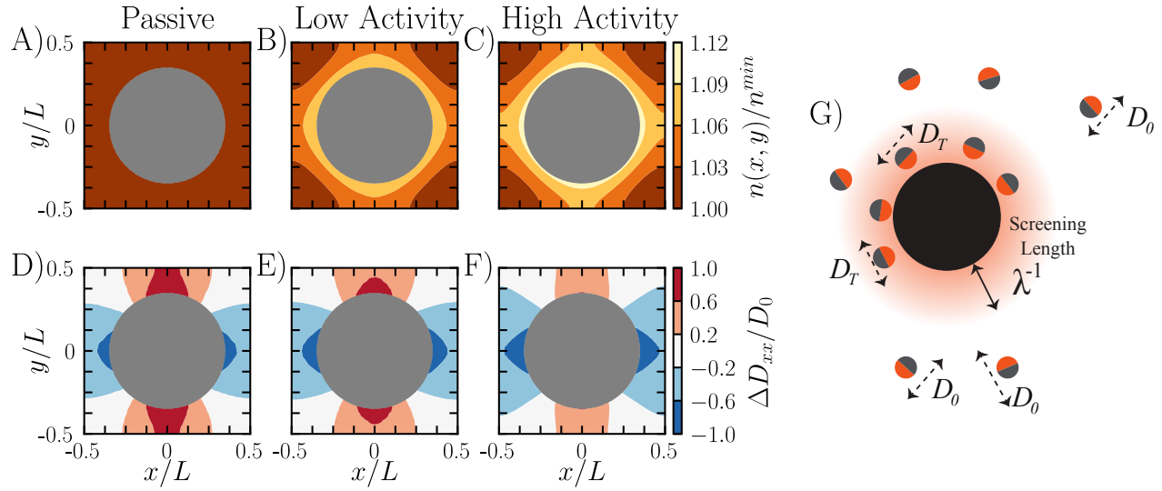
Fig. 4 Surface accumulation leads to slowdowns in scaled diffusivity. A-C) Local number density of particles for different activity parameters. As the activity increases in strength, the particles experience larger accumulation near the obstacle surface as shown through the contours. D-F) Pointwise diffusivity deviation along the x direction calculated numerically via dispersion theory (see Supplementary Information † for more details). The pointwise diffusivity deviation is \Delta D_{xx}/D_0 = (D_{xx}(x,y) - D_{\text{Model}})/D_0 . The pointwise diffusivity has a quadrupolar form due to particles getting trapped in the leading and trailing wakes of the obstacles. G) Cartoon demonstrating that ABPs within the boundary layer move with a reduced diffusivity compared to the ABPs in the bulk. Subplots A,D correspond to \ell/R = 0 and \delta^2/R^2 = N/A . Subplots B,E correspond to \ell/R = 1 and \delta^2/R^2 = 1 . Subplots C,F correspond to \ell/R = 10 and \delta^2/R^2 = 10 . All data collected for \phi = 0.38
