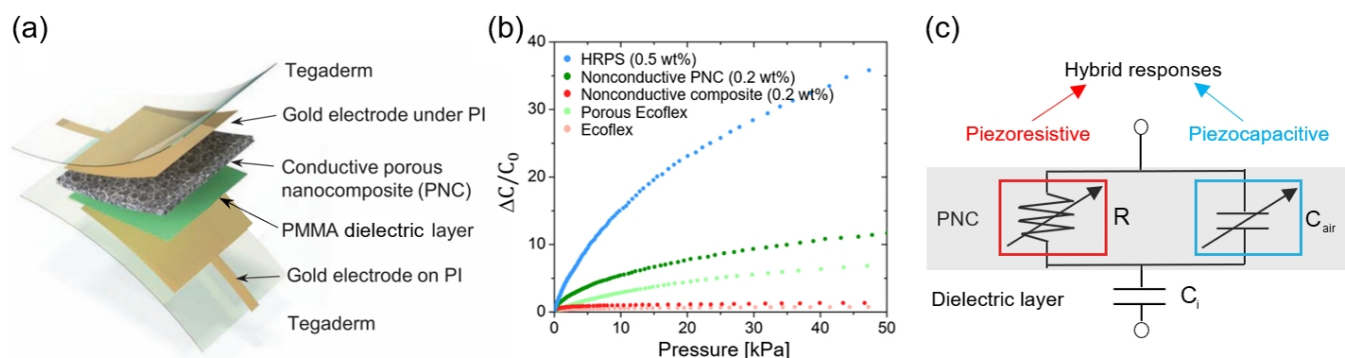
Fig. 1 (a) An exploded schematic of HRPS 24 . (b) HRPS is much more sensitive than conventional CPS 24 . (c) A simplified circuit model to represent the hybrid piezoresistive and piezocapacitive responses of HRPS. (a) & (b) reproduced from 24 with the permission of Wiley.
