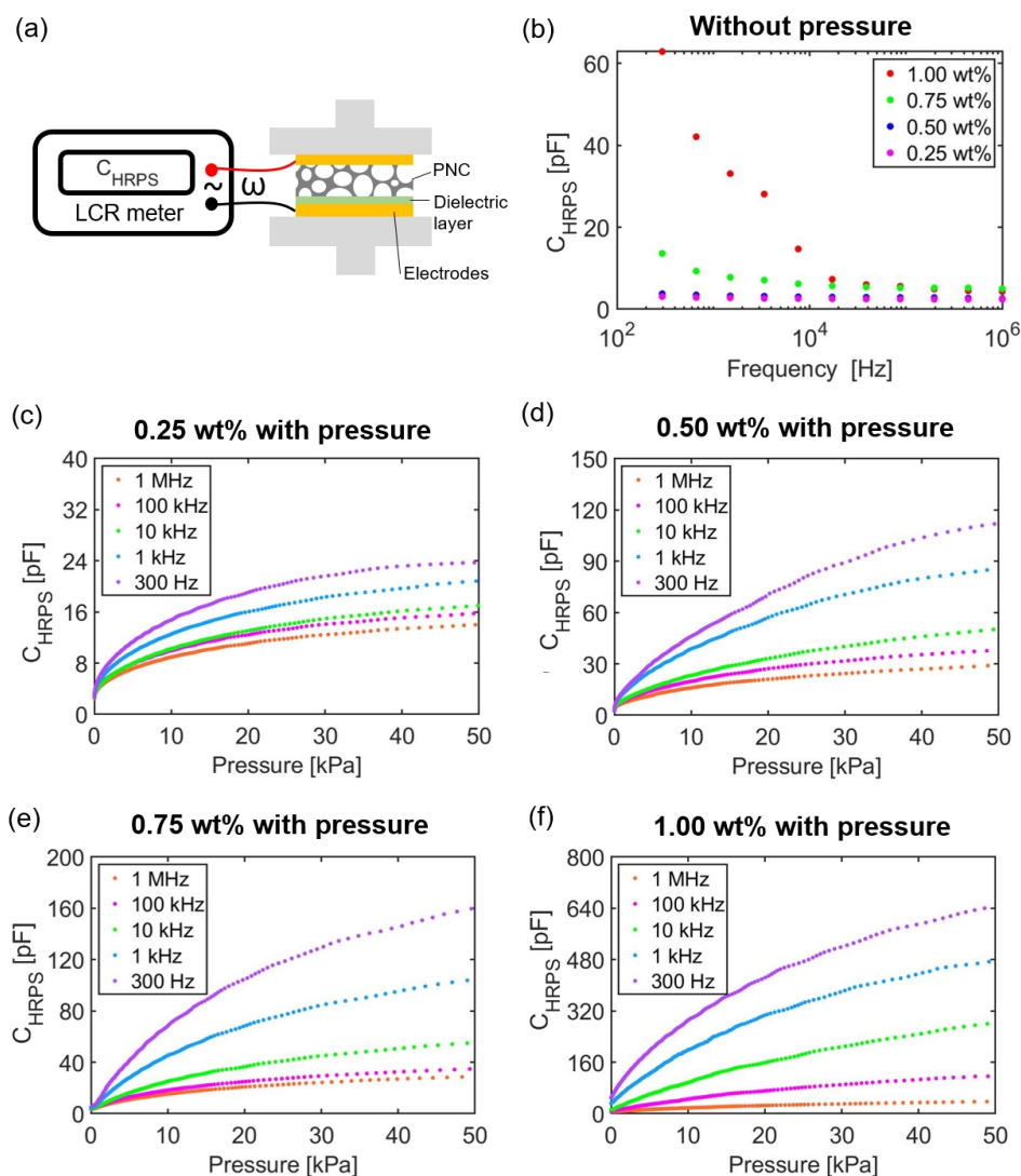
Fig. 2 (a) A schematic of the experimental setup for measuring the HRPS capacitance without and with applied pressure at different AC frequencies. (b) Frequency response of HRPS with different CNT doping ratios without any applied pressure. (c-f) Pressure response of HRPS under different AC frequencies (1 MHz, 100 kHz, 10 kHz, 1 kHz, and 300 Hz) with different CNT doping ratios: (c) 0.25 wt%, (d) 0.50 wt%, (e) 0.75 wt%, and (f) 1.00 wt%.
