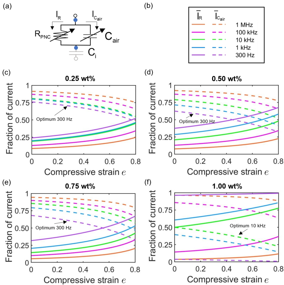
Fig. 6 (a) A schematic illustrating the current flowing through the piezoresistive branch ( I_R ) and the piezocapacitive branch ( I_{C_{air}} ) of the PNC. The two current fractions, \bar{I}_R + \bar{I}_{C_{air}} = 1 , meaning that there is a trade-off between the two. (b) Legends for the following plots. (c)-(f) The fractions of I_R (solid curves) and I_{C_{air}} (dashed curves) vs. the compressive strain at different AC frequencies for different CNT doping ratios: (c) 0.25 wt%, (d) 0.50 wt%, (e) 0.75 wt%, and (f) 1.00 wt%. The curve pairs closest to the equal divide of current correspond to the optimal frequency. In (c)-(d), the fraction of I_R is below 0.5 before compression but increases with compression whereas the fraction of I_{C_{air}} starts above 0.5 but decreases with compression. It indicates that the relative contribution of piezoresistivity enhances with compression but that of the piezocapacitivity diminishes with compression.
