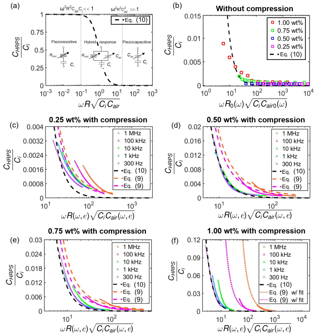
Fig. 4 (a) A master curve based on Eq (10) that can capture all three regimes - piezoresistive, hybrid, and piezocapacitive responses. (b) Frequency-only validation of the master curve. (c-f) Frequency and pressure validation of the master curve (black dashed curve). The colored dashed and dotted curves are based on Eq. (9). Note that as the compressive strain increases, the x axis \omega R \sqrt{C_i C_{air}} goes left.
