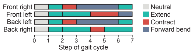
Fig. 7 7-Step Sequence for One Gait Cycle. The actuation sequence of each leg is shown at each step in the gait cycle, with actuation states of rest (neutral), extend, contract and forward bend combined in a series that produces forward walking.
