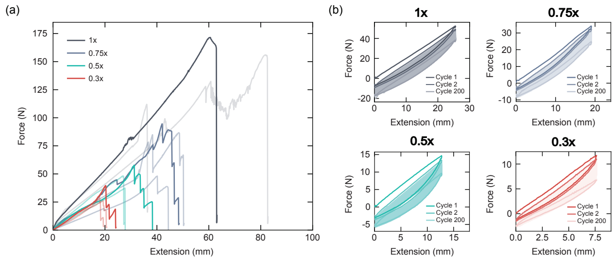
Fig. 2 Mechanical Characterization of HSAs. (a) Force versus extension data from tensile extension tests are shown for 1x, 0.75x, 0.5x, 0.3x HSAs. Data for three HSAs are provided for each scaling, with one plot from each set shown in bold color for improved visibility. (b) Force versus extension data from cyclic extension tests are shown for one HSA of each scale over 200 cycles at a rate of 10 mm/s for 1.0x and 0.75x HSAs and 1 mm/s for 0.5x and 0.3x HSAs. The 1st, 2nd, and 200th cycle are indicated in each plot.
