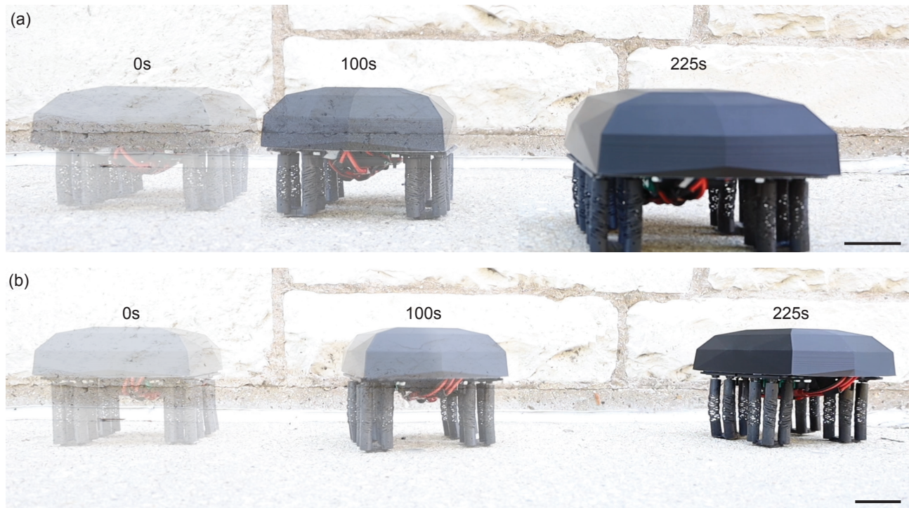
Fig. 6 Untethered Soft Robotic Quadrupeds. Untethered HSA-based soft robots constructed with the (a) 0.5x Legs and (b) Stilted 0.5x Legs are shown walking on a concrete sidewalk. Overlays of the quadrupeds are shown at 0 s, 100 s, and 225 s of the walking sequence. Stills are taken from Movie S4 in the ESI. Scale bars are 50 mm.
