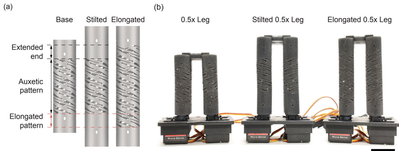
Fig. 3 HSA-Based Soft Robotic Legs. (a) Renderings of the base, stilted, and elongated HSAs used to construct the three HSA legs are shown, indicating the length of the extended ends (or stilts) and elongated auxetic pattern region. (b) The photograph shows the 0.5x Leg (left), Stilted 0.5x Leg (center), and Elongated 0.5x Leg (right) with the foot pointing upward. Scale bar is 20 mm.
