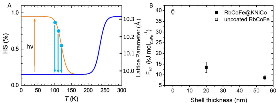
Fig. 4. (A) Schematic of the isothermal relaxation process. The sample is first cooled from room temperature (blue line) and the metastable HS state is established by light irradiation (yellow). The sample is then warmed to target temperatures (blue dots), where the decay of the HS state is monitored (blue arrows). (B) Activation energy vs shell thickness for the relaxation from the metastable HS state of RbCoFe-PBA as
